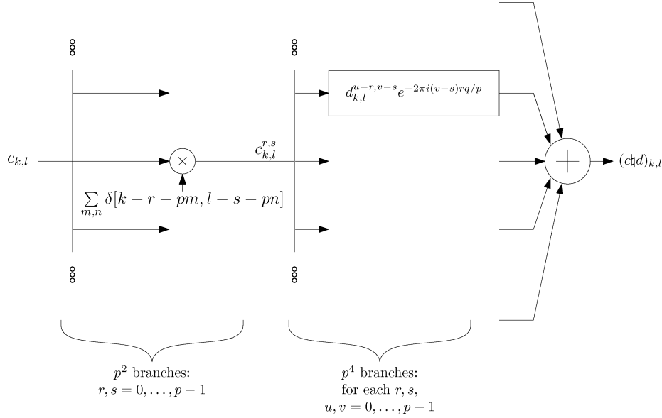
Fig. 7. A filter-bank realization of twisted convolution between c_{k,l} and d_{k,l} .
