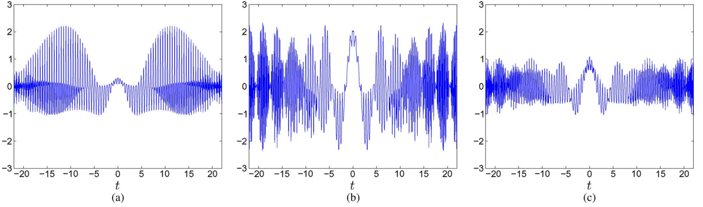
Fig. 5. Reconstructions of f(t) from its Gabor coefficients c_{k,l} . (a) Without processing c_{k,l} . (b) Consistent recovery, namely using d_{k,l} = (c * h_{\text{con}})_{k,l} as expansion coefficients. (c) Minimax-regret recovery, corresponding to d_{k,l} = (c * h_{\text{mx}})_{k,l} .
