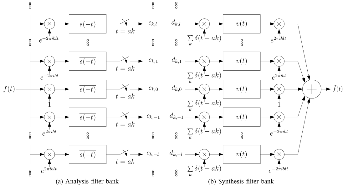
Fig. 1. Filter-bank representation of the Gabor transform (a) and of the inverse Gabor transform (b). (a) Analysis filter bank. (b) Synthesis filter bank.
