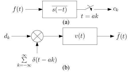
Fig. 2. Sampling (a) and reconstruction (b) with given filters.
