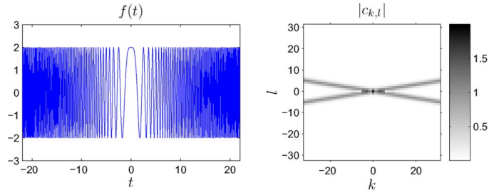
Fig. 4. A chirp signal and its Gaussian-window Gabor representation.
